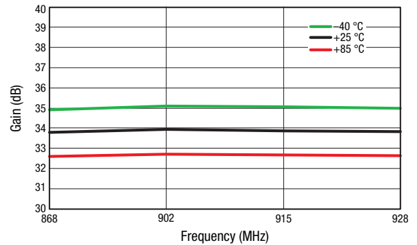
Figure 8. Transmit Path PA_IN to ANT1/ANT2 Gain vs Frequency Over Temperature
